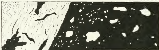
Fig. 33—Diagrammatic sketch showing ore body and schistose rock on hanging-wall, Garson mine, Sudbury area, Ontario, sixth level. Black represents sulphides. Width of face 12 feet.
